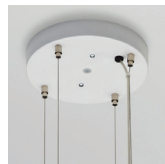
Plura 36 8" round canopy clear SPT with four 1/16" Ø steel cables
