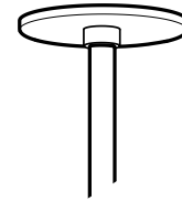
Rigid Suspension Canopy 8" Ø X 0.38"H
