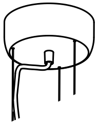
Corded Suspension Canopy 5" Ø X 2"H
